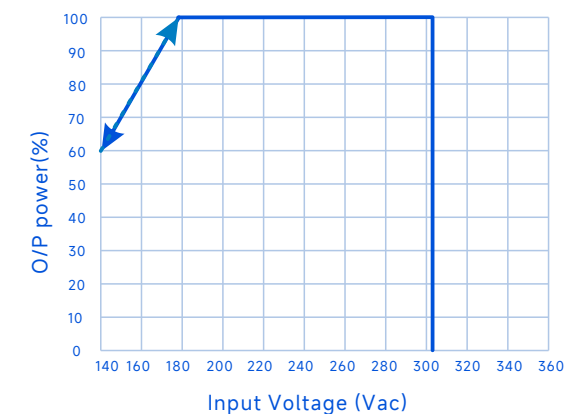
O/P Power Vs. Input Voltage
